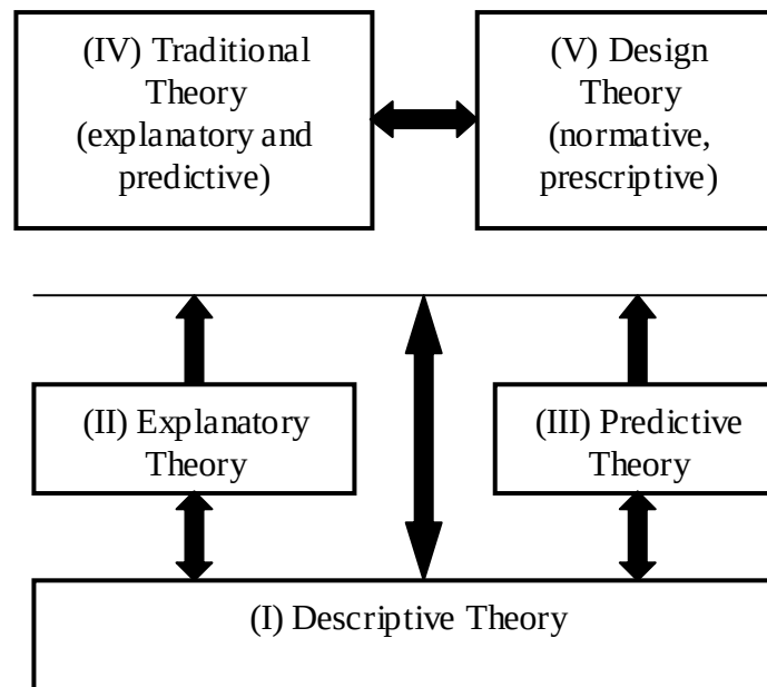
Figure 1: Interrelationships among theory types
